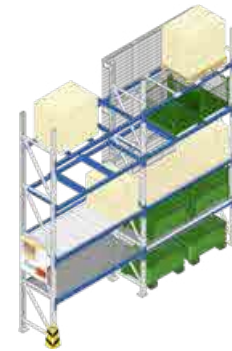
PR 350 longitudinal beam racking page D4
