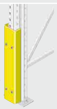
Upright protector with rubber buffer
